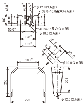
AW526、AW566、AW595
