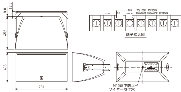
AW266/295-BK
