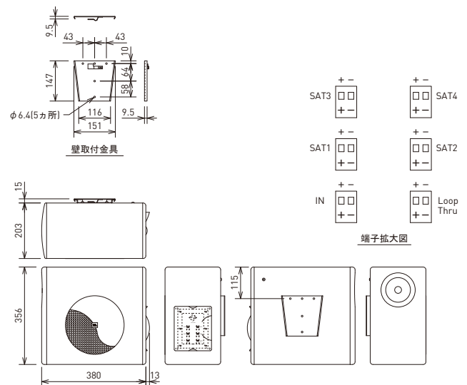
Control 50S/T-WH
