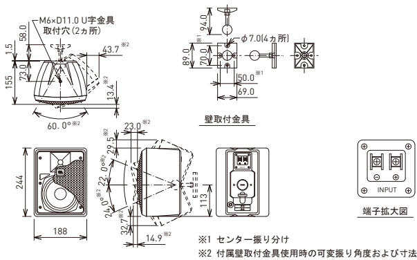
Control 25-1-WH
