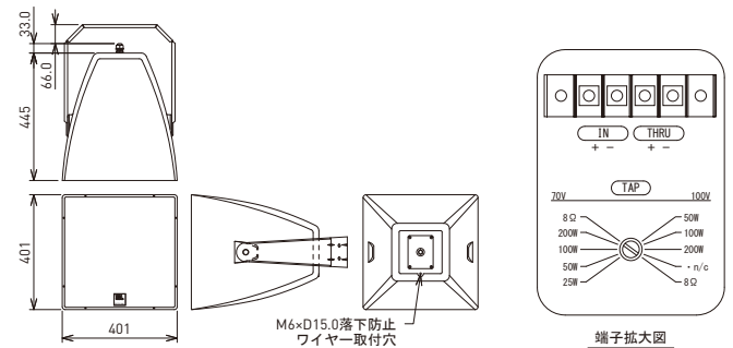
AWC129-BK
