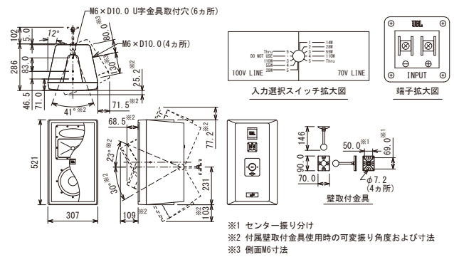
Control 29AV-1-WH
