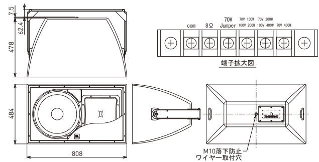
AW526/566/595-BK
