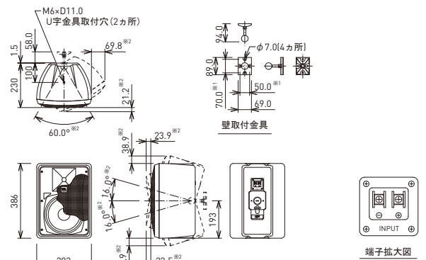
Control 28-1-WH
