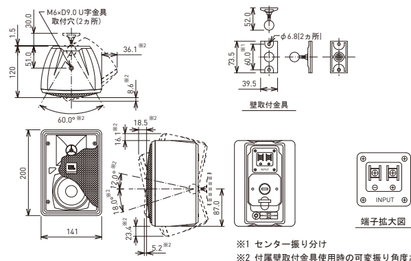
Control 23-1-WH
