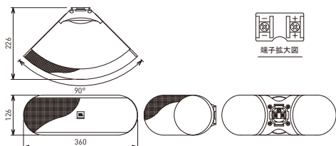
Control CRV-WH
